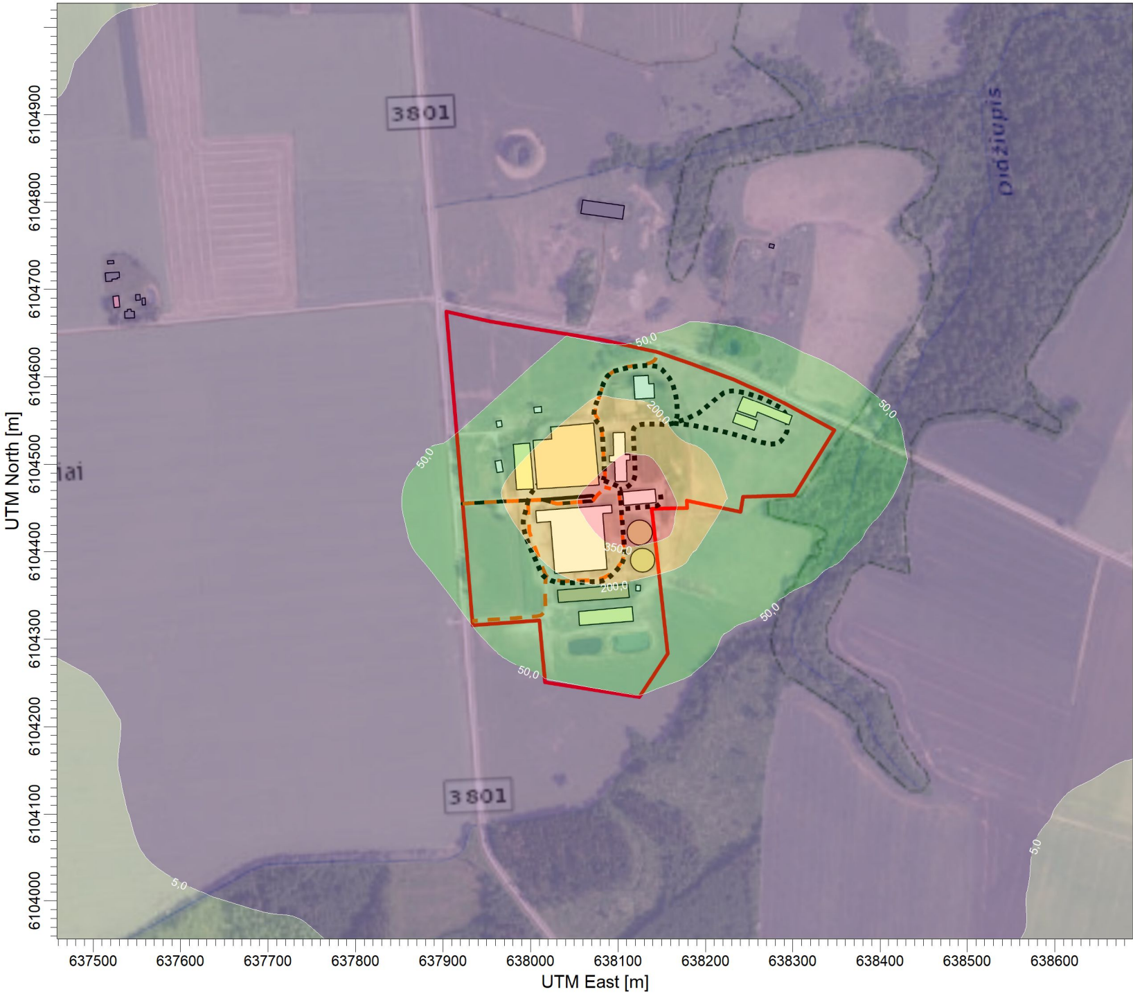
PLOT FILE OF 98.50TH PERCENTILE 1-HR VALUES FOR SOURCE GROUP: ALL Max: 499.5 [ug/m^3] at (638139,56, 6104448,13)
