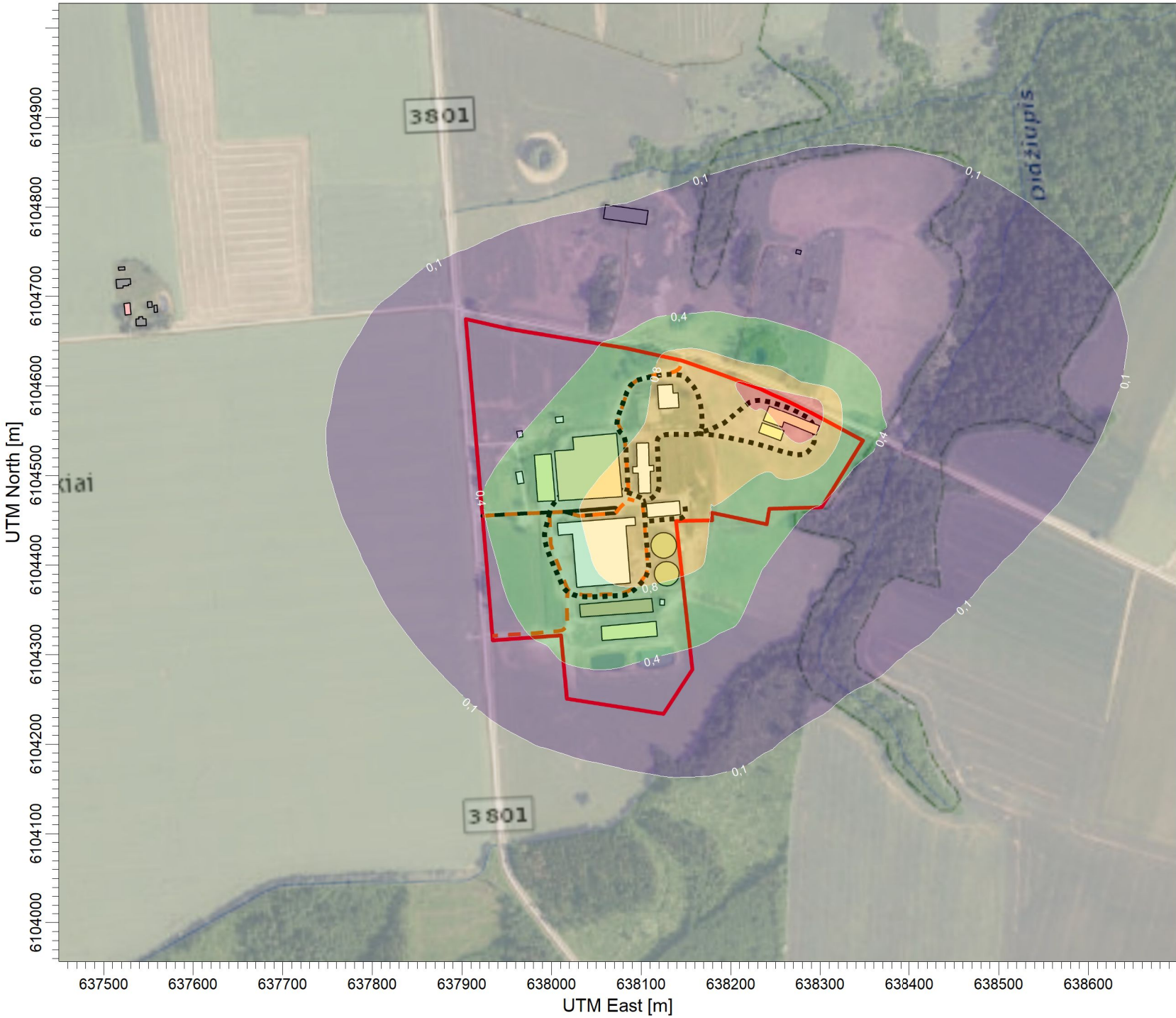
PLOT FILE OF ANNUAL VALUES AVERAGED ACROSS 5 YEARS FOR SOURCE GROUP: UV Max: 1,6 [ug/m^3] at (638283,01, 6104573,57)
