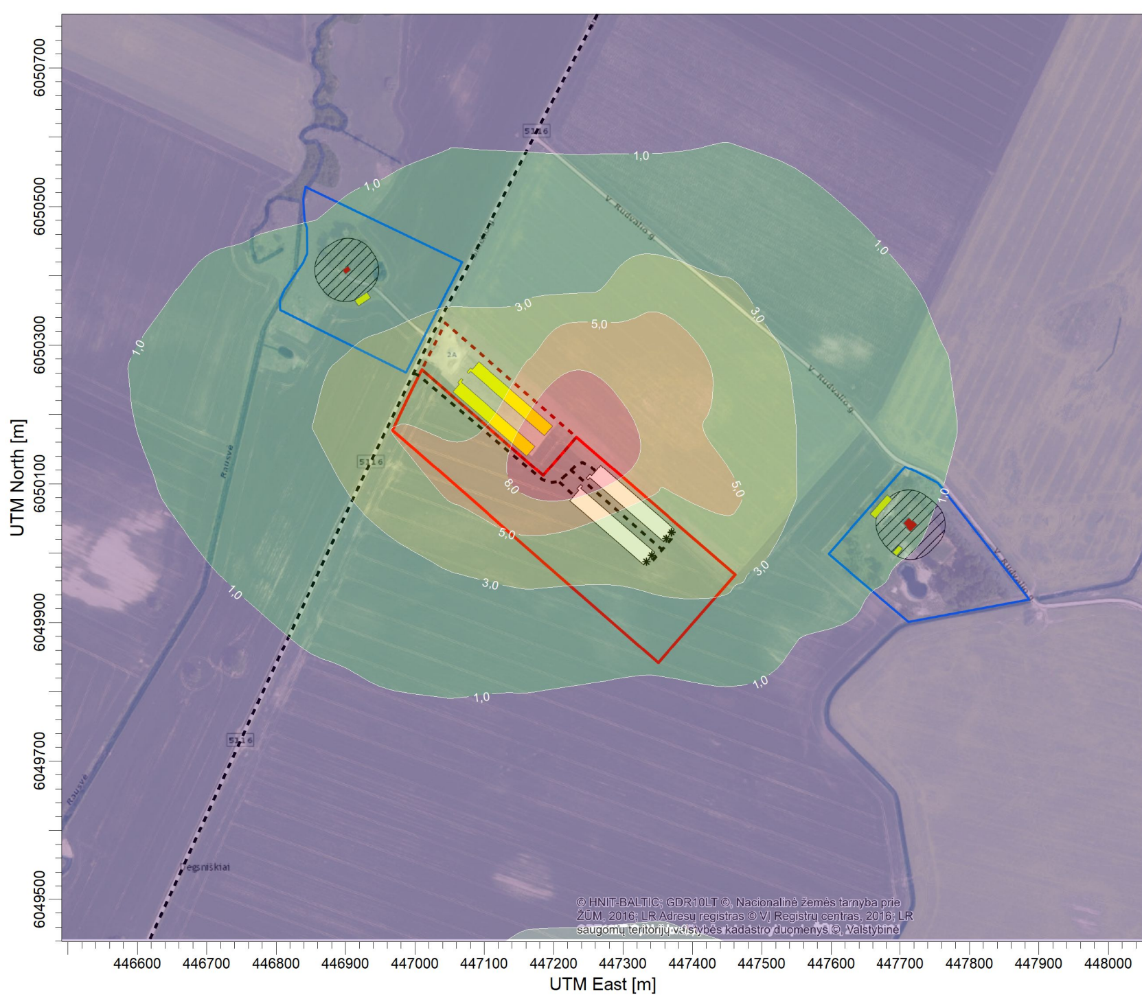
PLOT FILE OF 98.08TH PERCENTILE 1-HR VALUES FOR SOURCE GROUP: ALL Max: 14,6 [OU/M**3] at (447253,30, 6050181,72)
