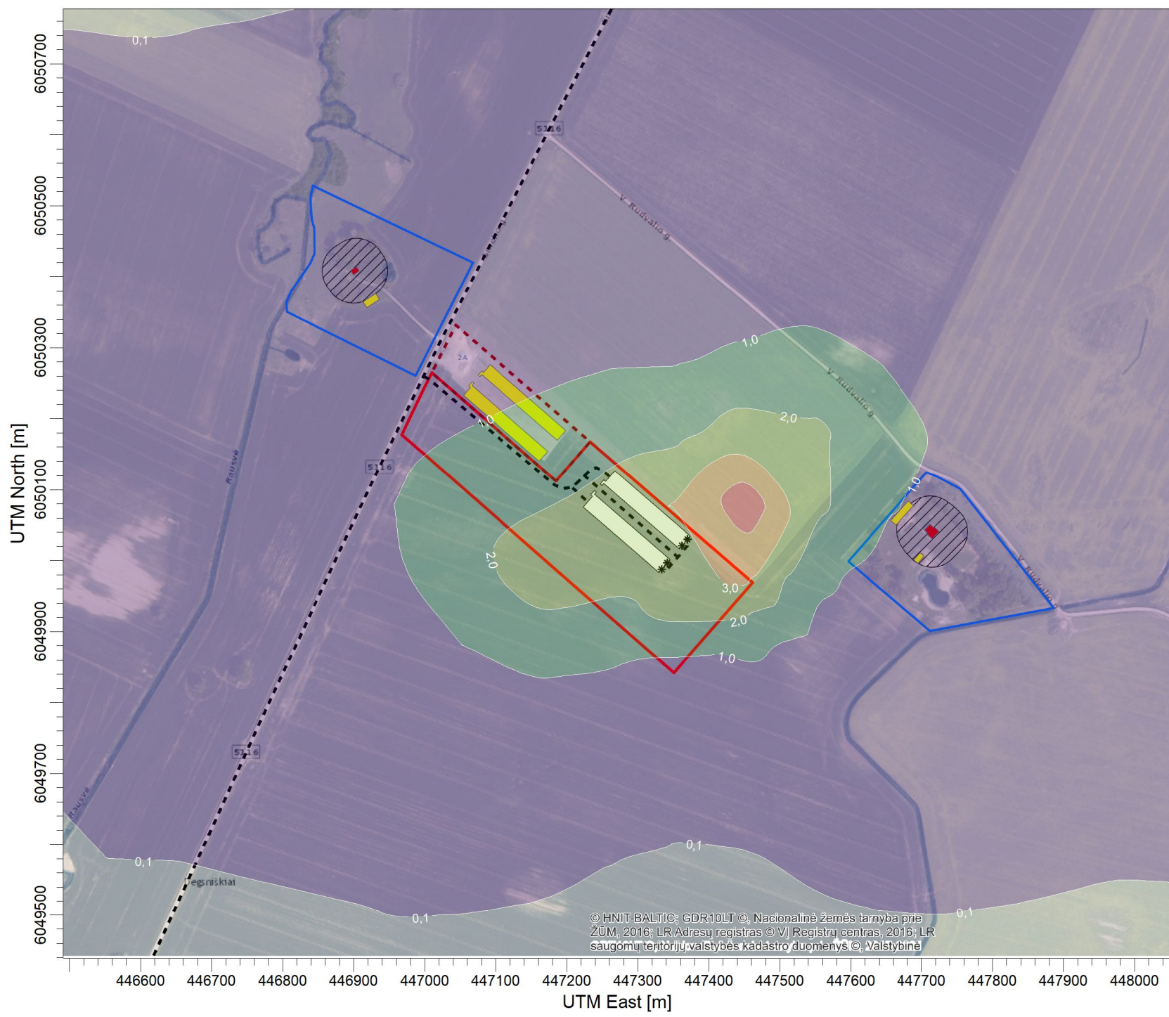
PLOT FILE OF 98.08TH PERCENTILE 1-HR VALUES FOR SOURCE GROUP: PUV Max: 4,7 [OJ/M**3] at (447453,30, 6050081,72)
