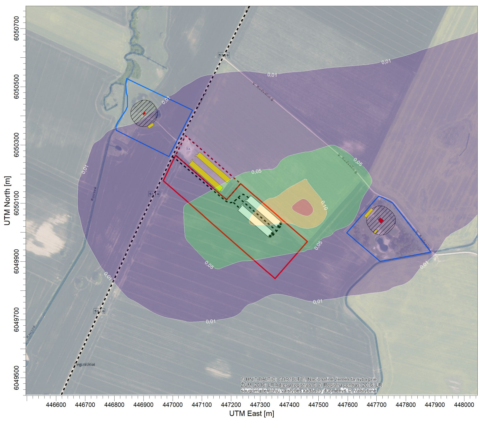
PLOT FILE OF ANNUAL VALUES AVERAGED ACROSS 5 YEARS FOR SOURCE GROUP: PUV Max: 0,18 [ug/m^3] at (447453,30, 6050081,72)
