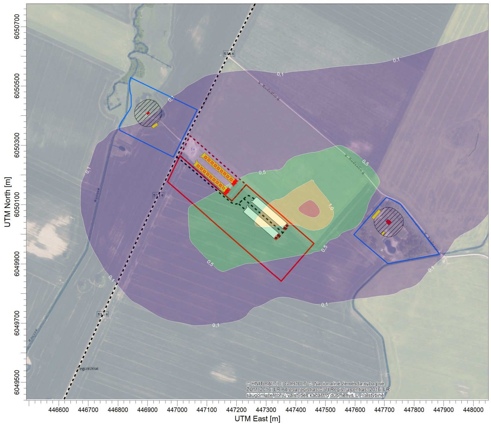
PLOT FILE OF ANNUAL VALUES AVERAGED ACROSS 5 YEARS FOR SOURCE GROUP: PUV Max: 1,8 [ \mu\text{g}/\text{m}^3 ] at (447453,30, 6050081,72)
