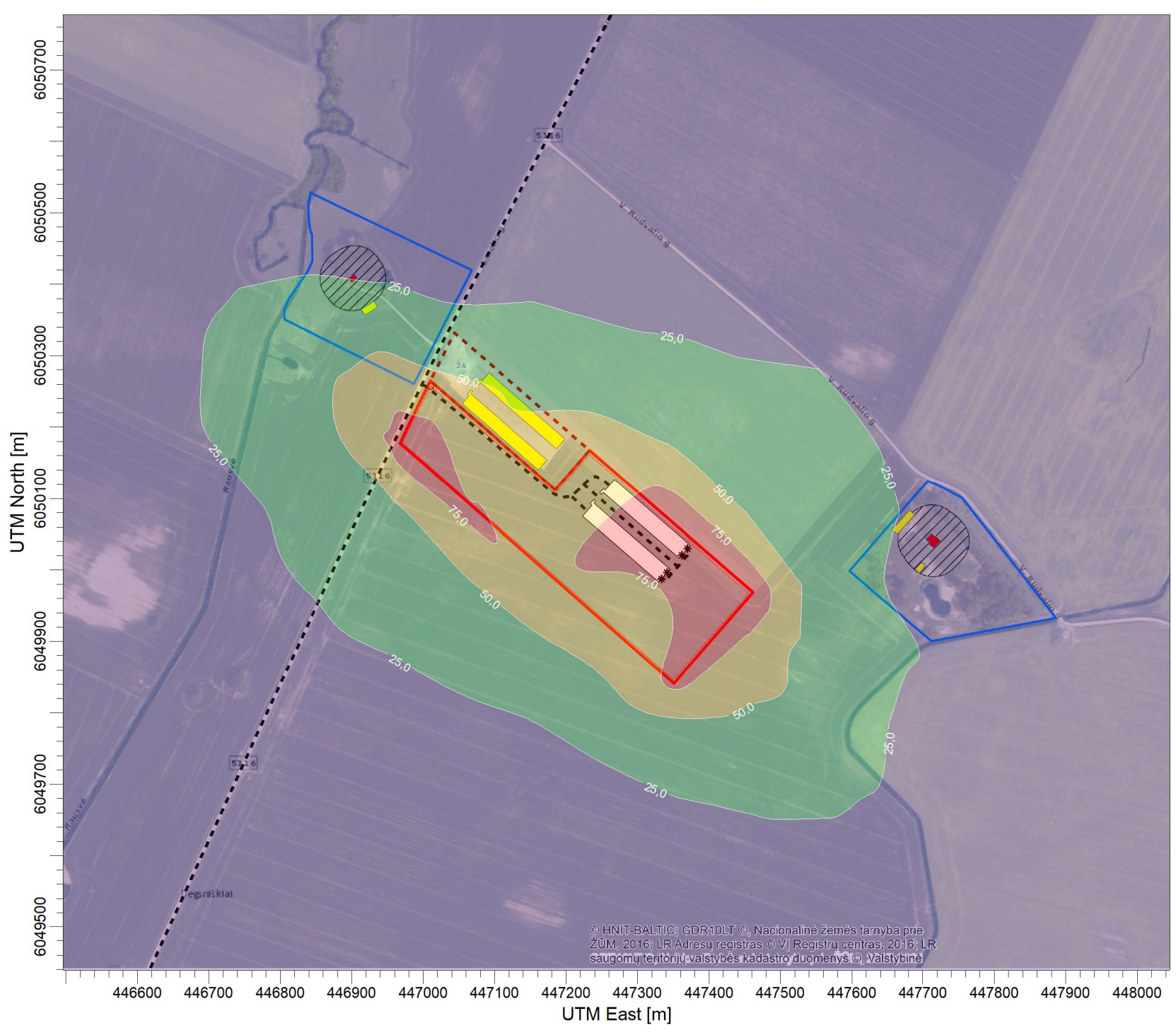
PLOT FILE OF HIGH 1ST HIGH 8-HR VALUES FOR SOURCE GROUP: PUV Max: 91,1 [ug/m 3 ] at (446967,28, 6050176,70)
