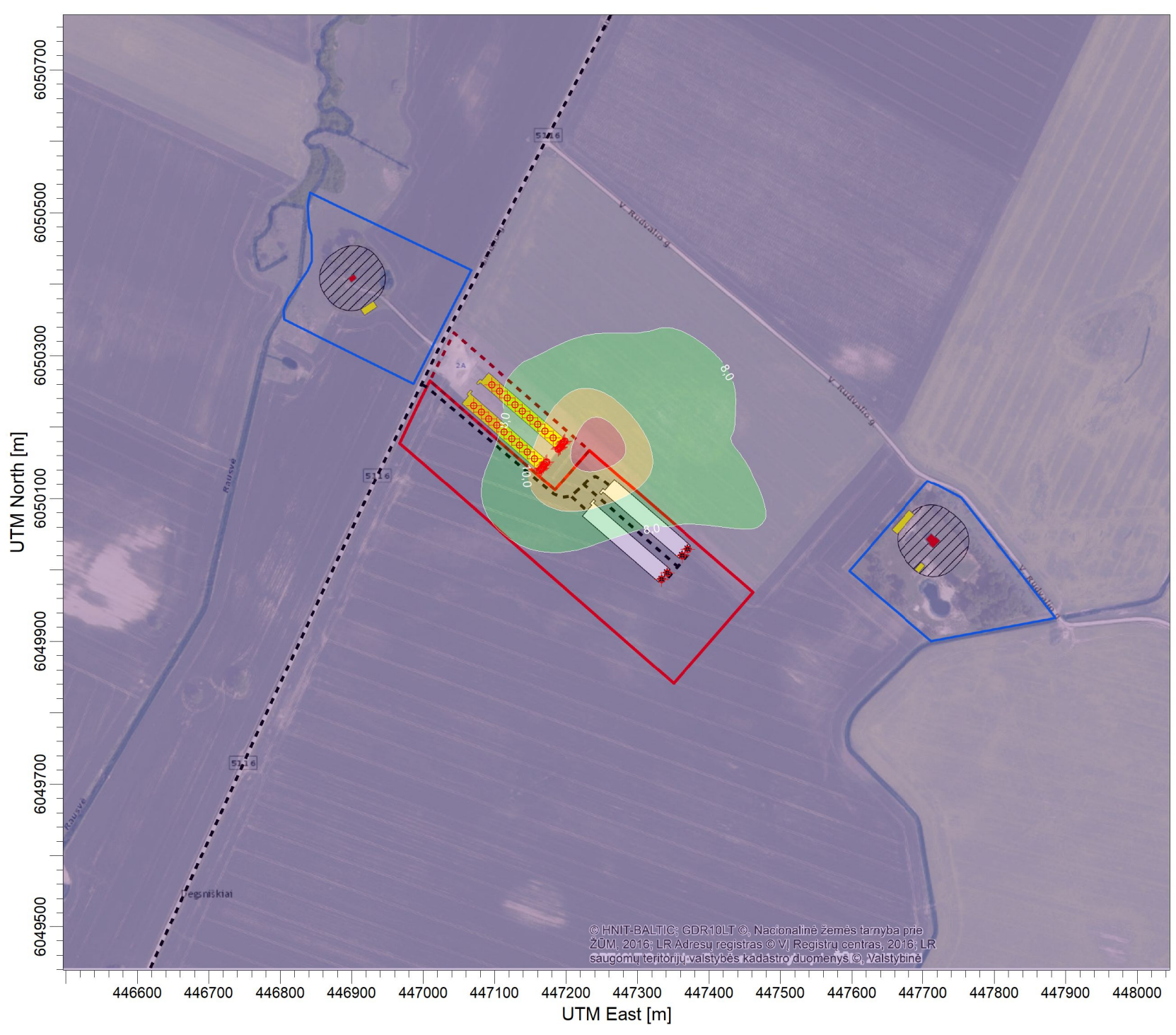
PLOT FILE OF ANNUAL VALUES AVERAGED ACROSS 5 YEARS FOR SOURCE GROUP: ALL Max: 13,6 [ug/m^3] at (447253,30, 6050181,72)
