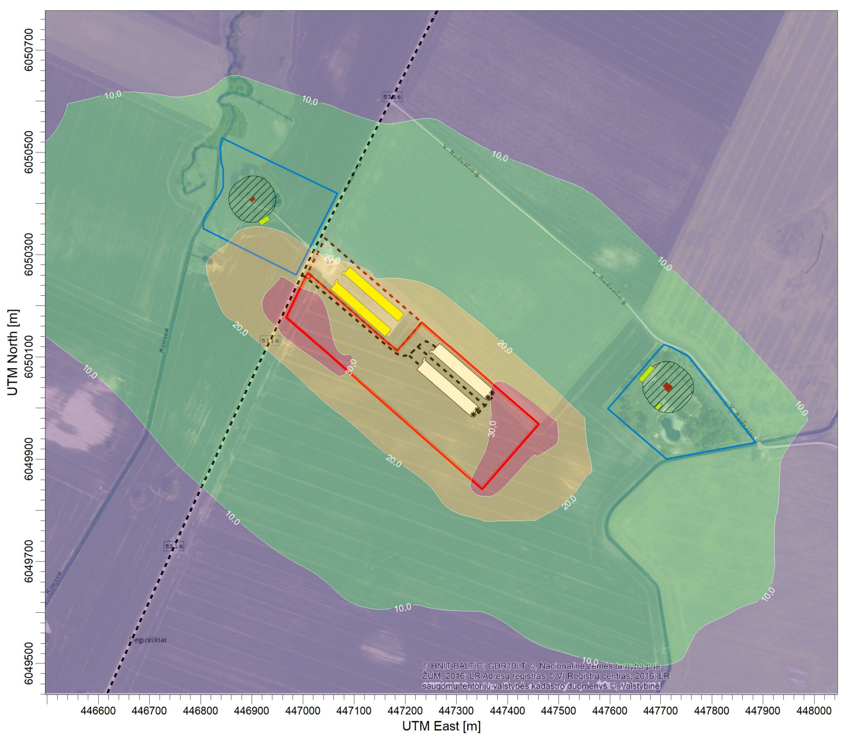
PLOT FILE OF 99.80TH PERCENTILE 1-HR VALUES FOR SOURCE GROUP: ALL Max: 38,5 [ug/m^3] at (446967,28, 6050176,70)
