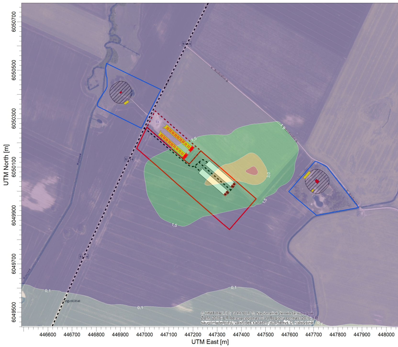
PLOT FILE OF 90.40TH PERCENTILE 24-HR VALUES FOR SOURCE GROUP: PUV Max: 4,4 [ug/m^3] at (447453,30, 6050081,72)
