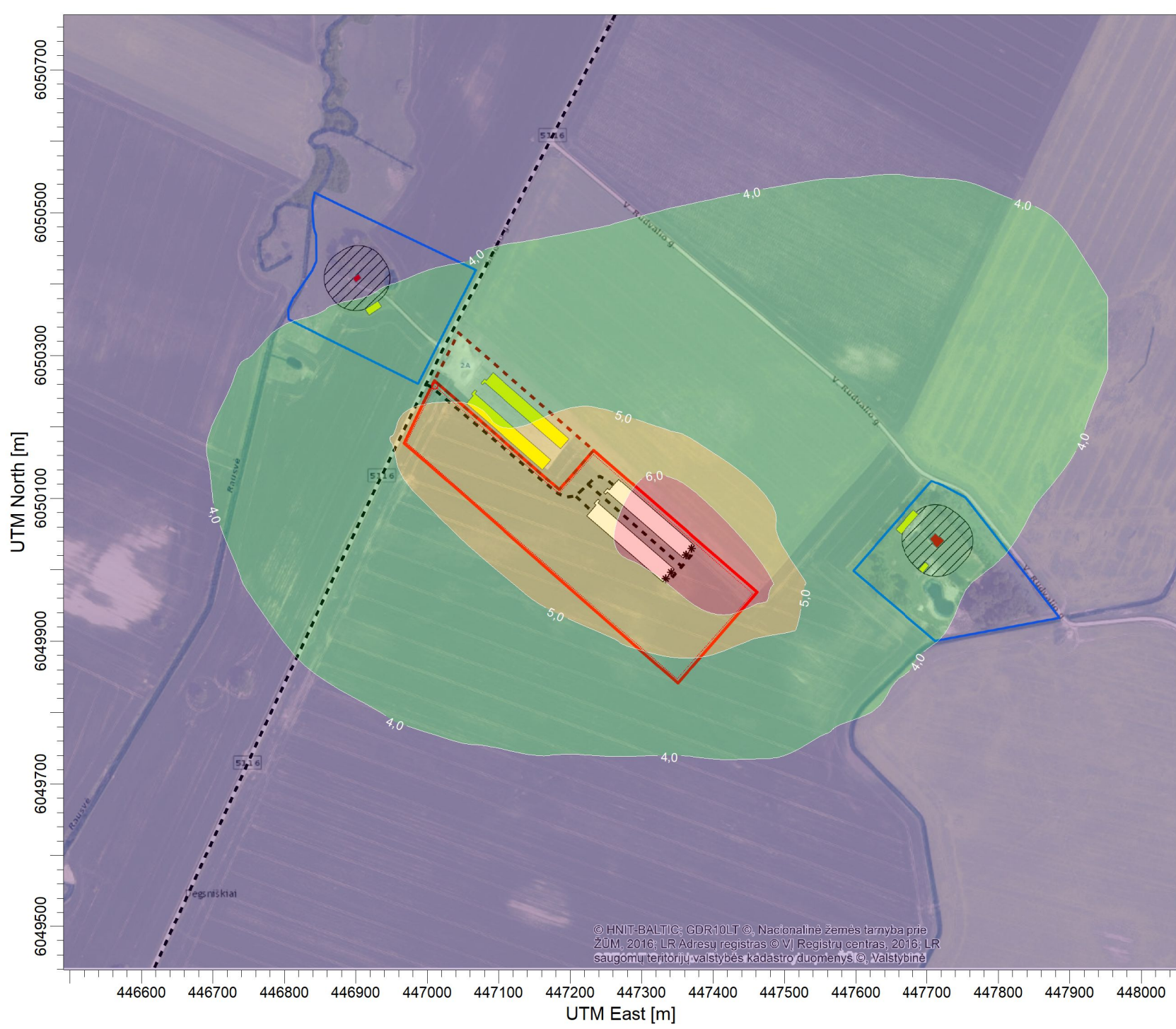
PLOT FILE OF ANNUAL VALUES AVERAGED ACROSS 5 YEARS FOR SOURCE GROUP: ALL Max: 6,8 [ug/m^3] at (447353,30, 6050081,72)
