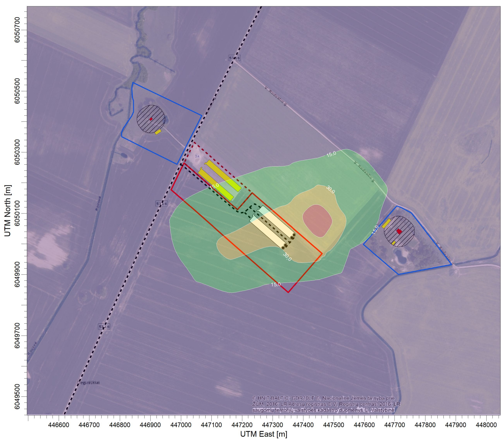
PLOT FILE OF 98.50TH PERCENTILE 1-HR VALUES FOR SOURCE GROUP: PUV Max: 59,7 [ug/m^3] at (447453,30, 6050081,72)
