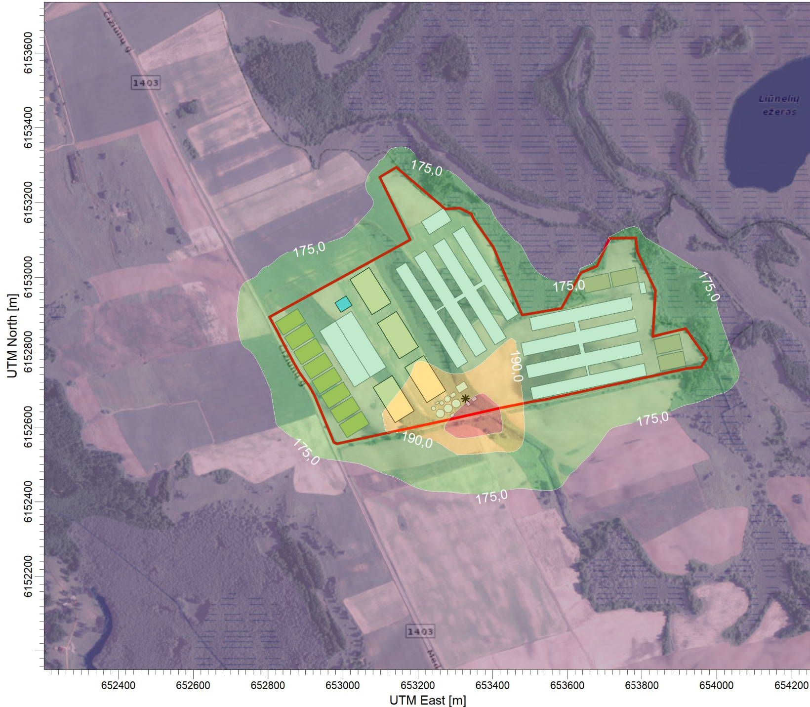
PLOT FILE OF HIGH 1ST HIGH 8-HR VALUES FOR SOURCE GROUP: ALL Max: 215.6 [ug/m 3 ] at (653306,97, 6152599,97)
