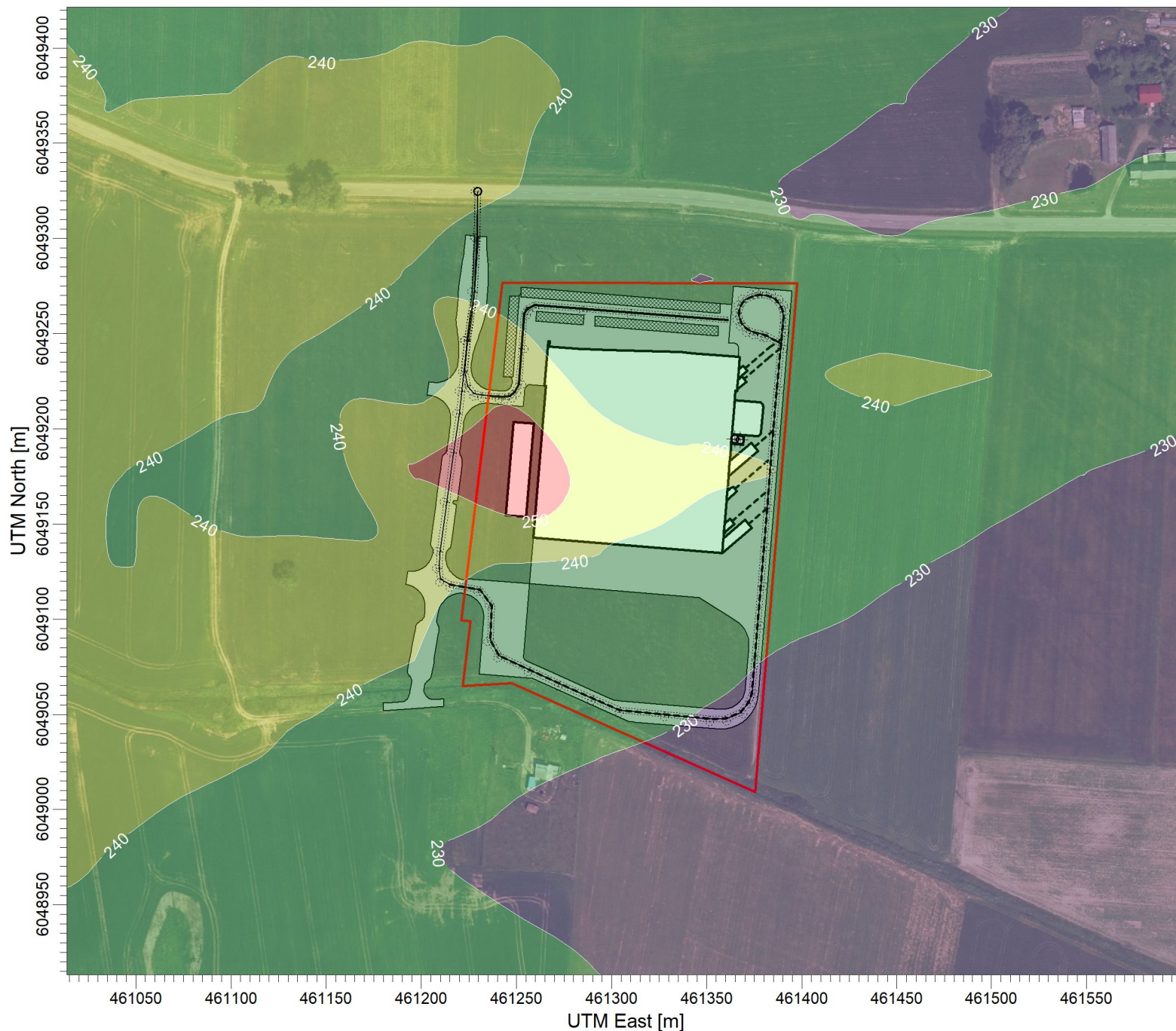
PLOT FILE OF HIGH 1ST HIGH 8-HR VALUES FOR SOURCE GROUP: ALL Max: 261,3 [ug/m^3] at (461246,39, 6049178,22)
