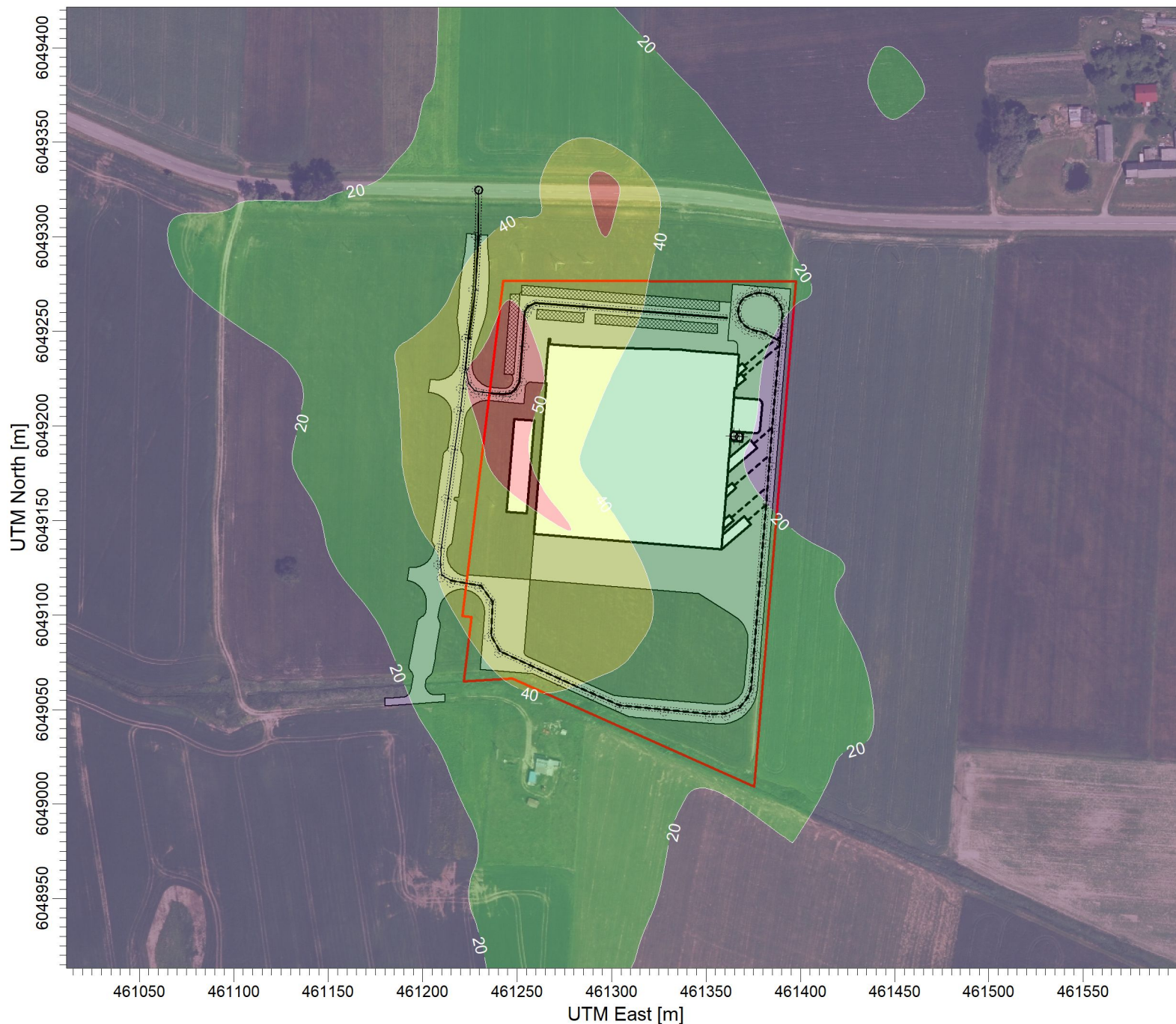
PLOT FILE OF HIGH 1ST HIGH 8-HR VALUES FOR SOURCE GROUP: PŪV Max: 56,0 [ug/m^3] at (461246,39, 6049228,22)
