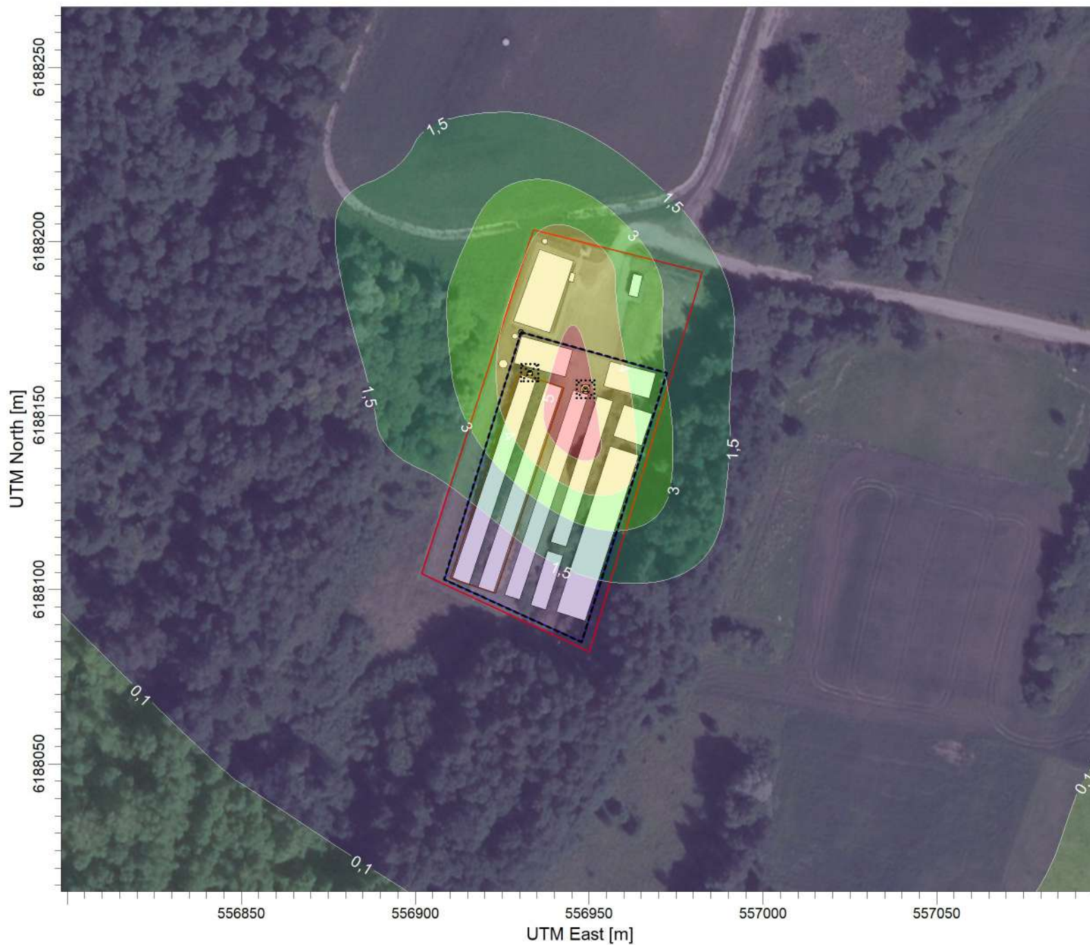
PLOT FILE OF 90.40TH PERCENTILE 24-HR VALUES FOR SOURCE GROUP: PUV Max: 5,7 [ \mu\text{g}/\text{m}^3 ] at (556946,24, 6188144,19)
